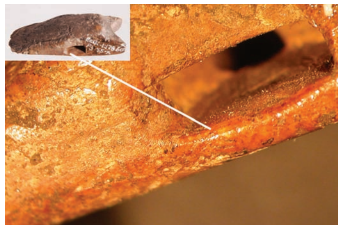
FIG. 4. Magnified (10×) view of a line hole on a line fastener showing polished edge.
