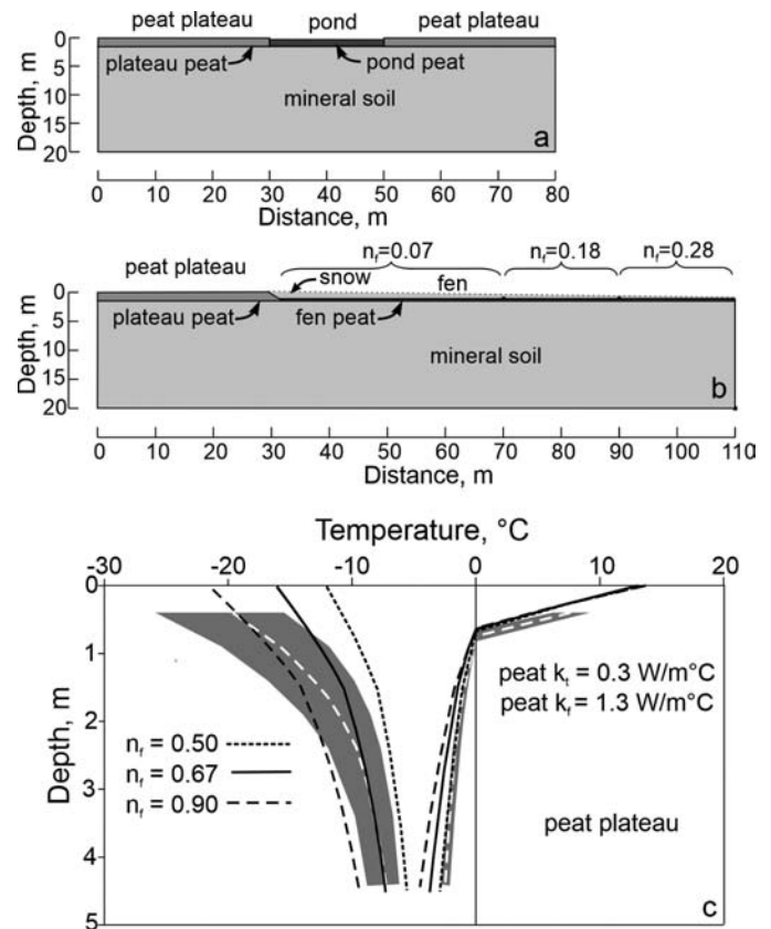
FIG. 7. Modelling cross sections used with TEMP/W. a) A single pond on a peat plateau. The pond is 30 cm deep and underlain by pond peat, the peat plateau underlain by plateau peat. Both peat types are underlain by mineral soil (silty sand—see Table 2 for thermal properties). Pond sizes of 10, 20, and 40 m are modelled. b) A fen adjoining a peat plateau. Fen peat is 30 cm thick. N -factor zones simulating decreasing snow depths away from the peat plateau edge are indicated. All material properties and conditions are listed in Table 2. Both models include a geothermal heat flux of 0.05 \text{ W/m}^2 . c) Comparison of the Fletcher Lake site peat plateau ground temperature record with modelling. The range of annual extremes, 2008–18 (shown in grey), and the mean for this time interval (white dashed line) are compared with the modelled mean annual extremes for different freezing n -factors. The thawed n -factor used is 0.90.
